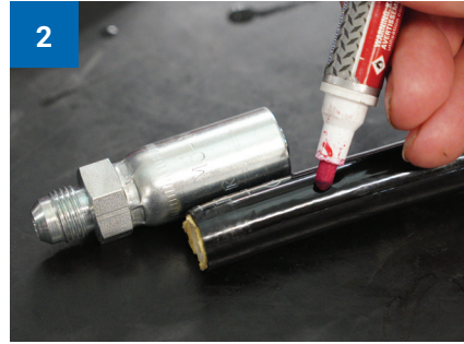
Mark insertion depth.
