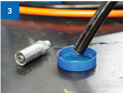
Lightly lubricate hose end to ease coupling insertion
