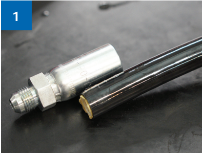
Establish hose insertion depth using the coupling you're going to swage.
